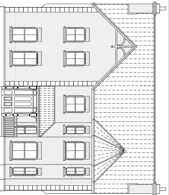
FRONT ELEVATION
